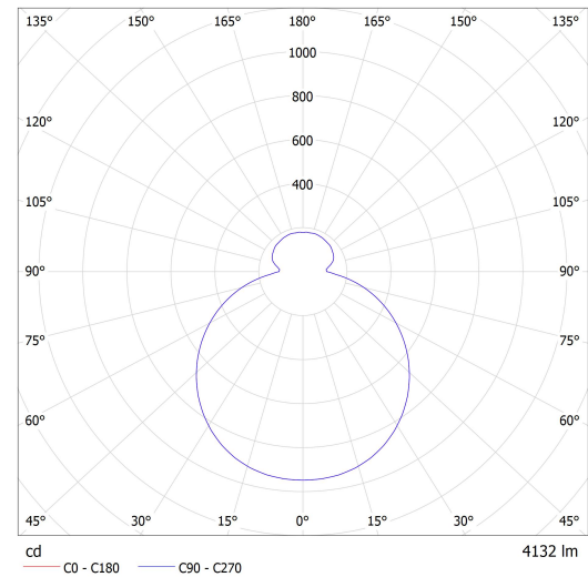
Lucis PS13.K4.Z600 ZERO LED / LDC (Polar)
