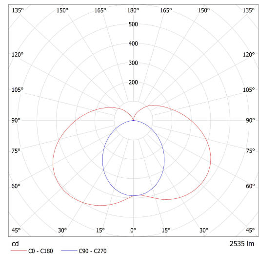
Luminaire: Lucis AU3.L1.600.X AULA LED Lamps: 1 x LED G6
