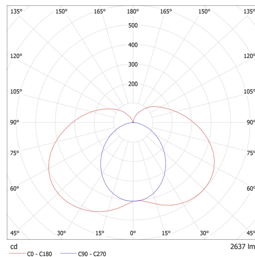
Luminaire: Lucis AU3.L2.600.X AULA LED Lamps: 1 x LED G6
