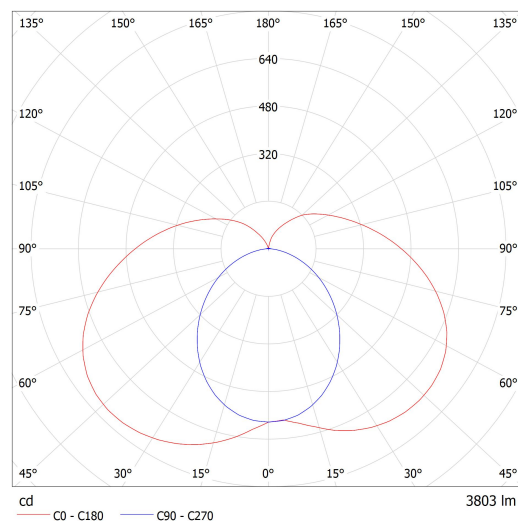
Luminaire: Lucis AU3.L1.900.X AULA LED Lamps: 1 x LED G6
