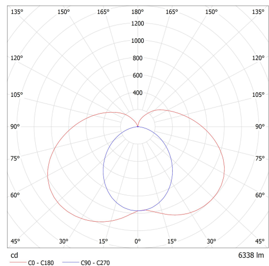
Luminaire: Lucis AU3.L1.1500.X AULA LED Lamps: 1 x LED G6
