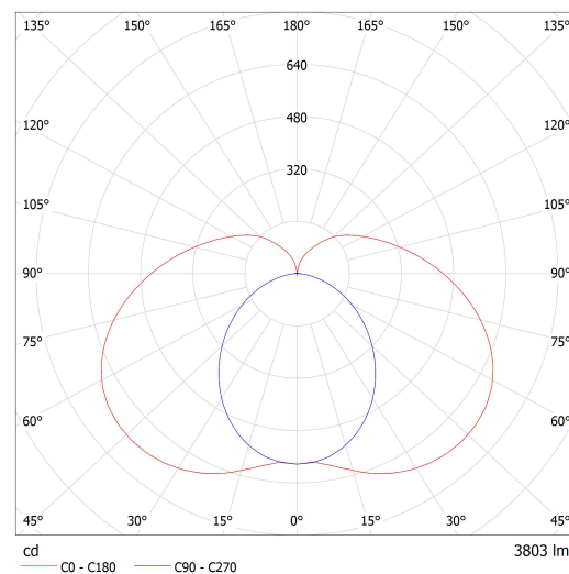
Luminaire: Lucis AU1.L1.900.X AULA LED Lamps: 1 x LED G6
