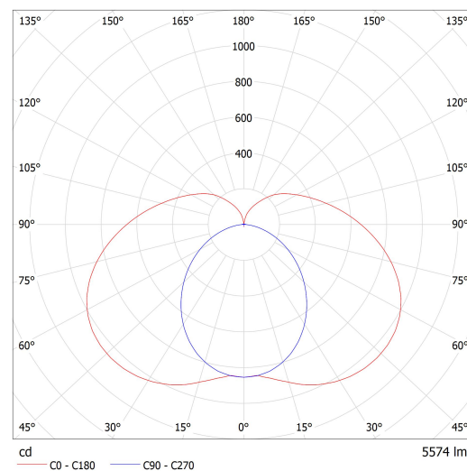
Luminaire: Lucis AU1.L2.1200.X AULA LED Lamps: 1 x LED G6
