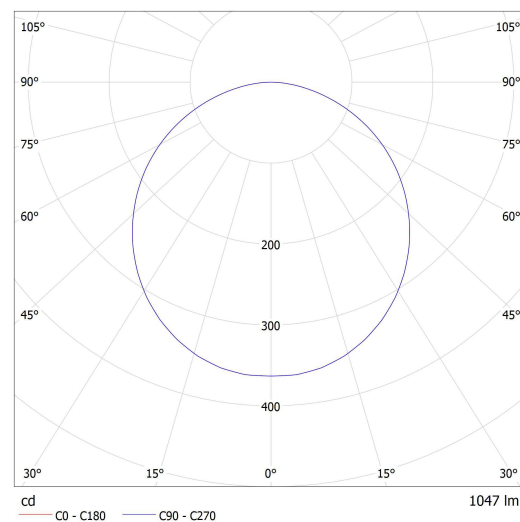
Lucis ZK.K2.E120.X ELIOS LED / LDC (Polar)
