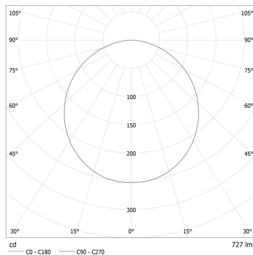
Lucis ZK.K3.E120.X ELIOS LED / LDC (Polar)
