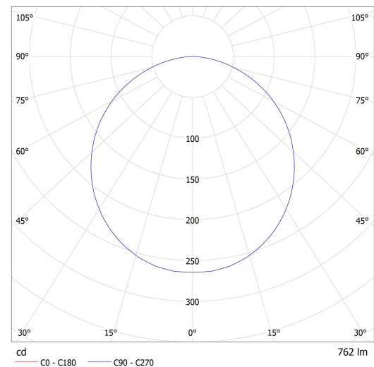
Lucis ZK.K4.E120.X ELIOS LED / LDC (Polar)
