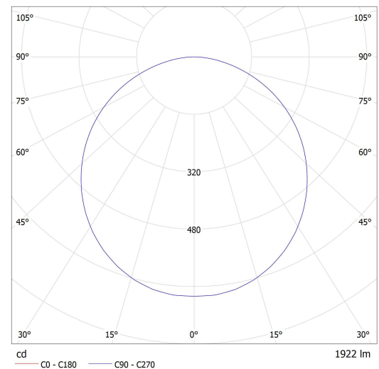
Lucis ZK3.K1.E220.X ELIOS LED / LDC (Polar)
