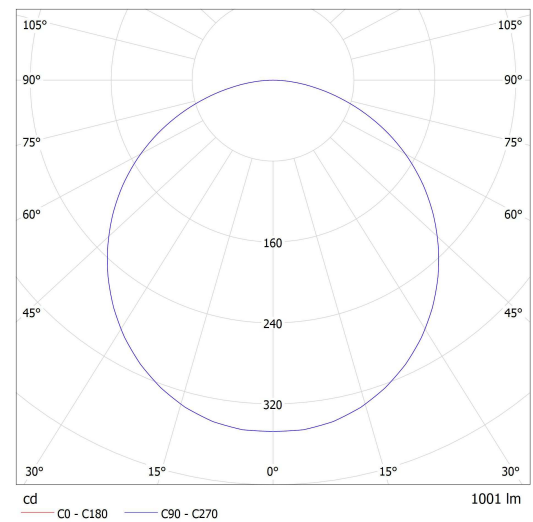
Lucis S7.K1.E120.X ELIOS LED / LDC (Polar)
