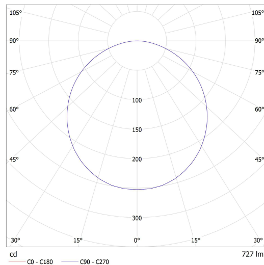
Lucis S7.K3.E120.X ELIOS LED / LDC (Polar)
