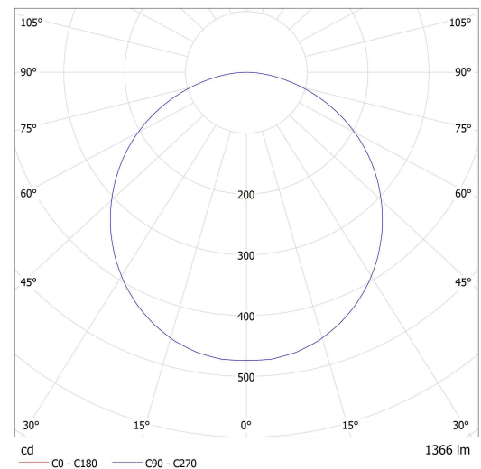
Lucis S7.K3.E220.X ELIOS LED / LDC (Polar)
