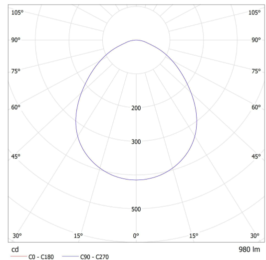
Lucis ZK.K1.J1.X JUNO LED / LDC (Polar)
