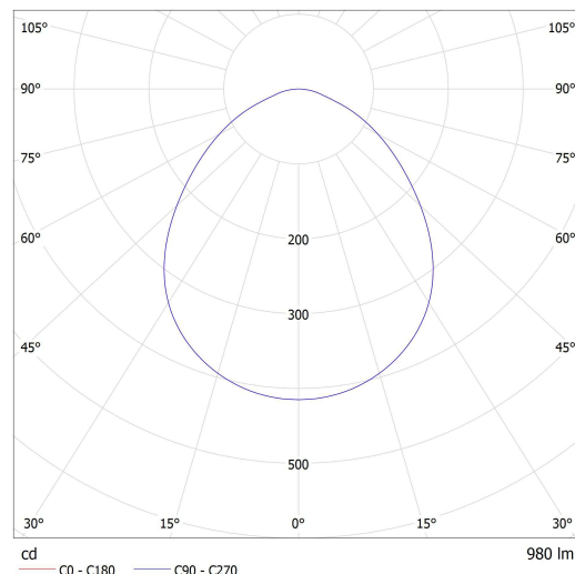
Lucis ZK.K1.J1.X JUNO LED / LDC (Polar)
