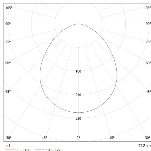
Lucis ZK.K3.J1.X JUNO LED / LDC (Polar)
