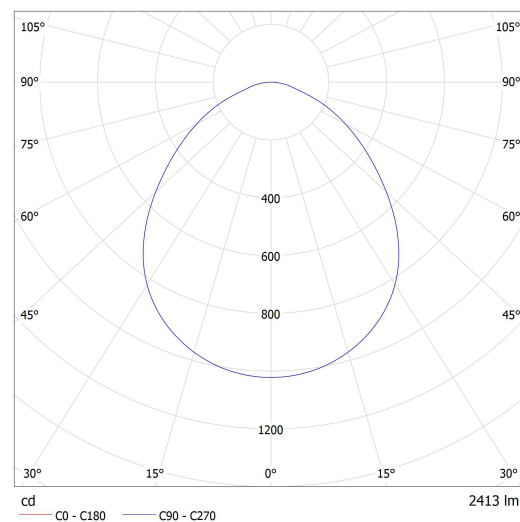
Lucis ZK.K3.J3.X JUNO LED / LDC (Polar)
