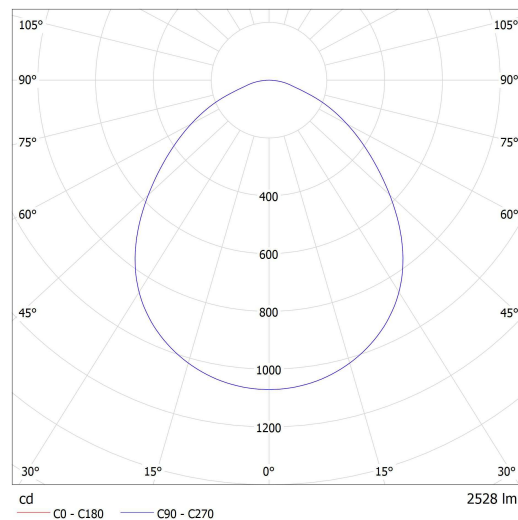
Lucis ZK.K4.J3.X JUNO LED / LDC (Polar)
