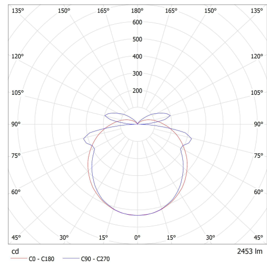
Luminaire: Lucis S3.L2W MAIA LED Lamps: 1 x LED G5
