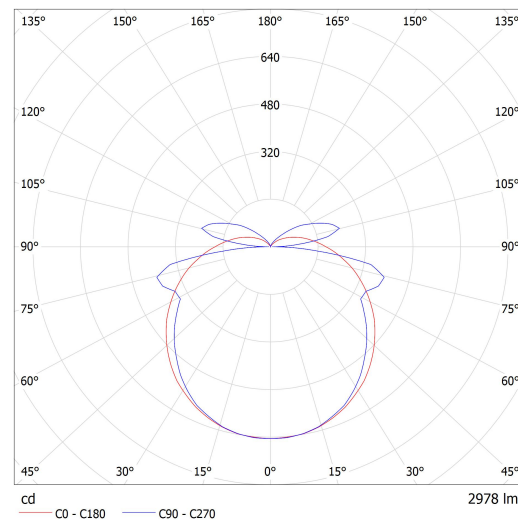
Luminaire: Lucis S3.L1W PA MAIA LED Lamps: 1 x LED G6
