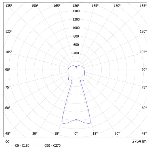
Luminaire: Lucis ZKS.L1A.M320 MAIA LED Lamps: 1 x LED G6
