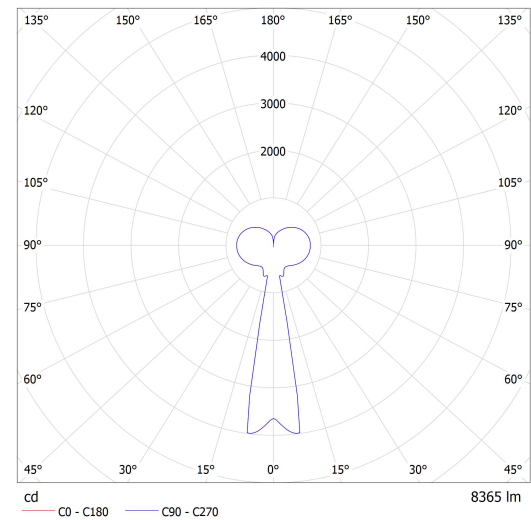
Luminaire: Lucis ZKS.L2A.M620 MAIA LED Lamps: 1 x LED G6
