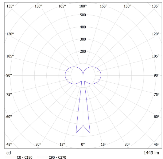
Luminaire: Lucis ZKS.L2A.M380 MAIA LED Lamps: 1 x LED G6
