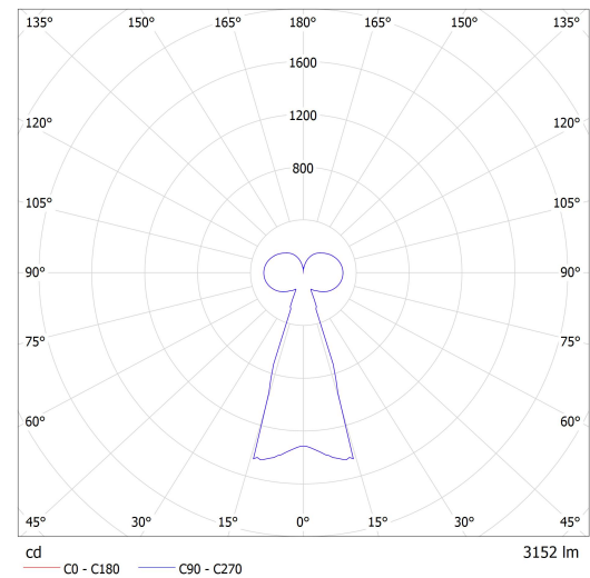
Luminaire: Lucis ZKS.L1A.M320 PA MAIA LED Lamps: 1 x LED G6
