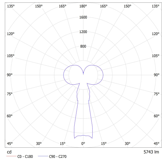
Luminaire: Lucis ZKS.L1A.M500 PA MAIA LED Lamps: 1 x LED G6
