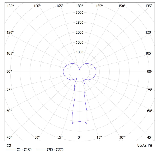
Luminaire: Lucis ZKS.L1A.M620 PA MAIA LED Lamps: 1 x LED G6
