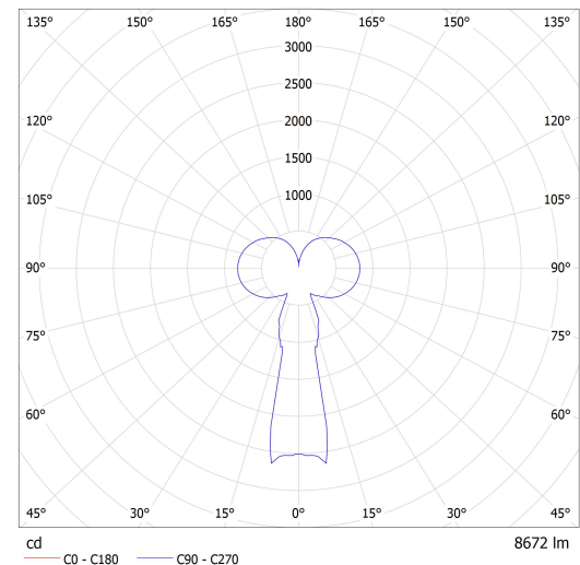
Luminaire: Lucis ZKS.L1A.M620 PA MAIA LED Lamps: 1 x LED G6
