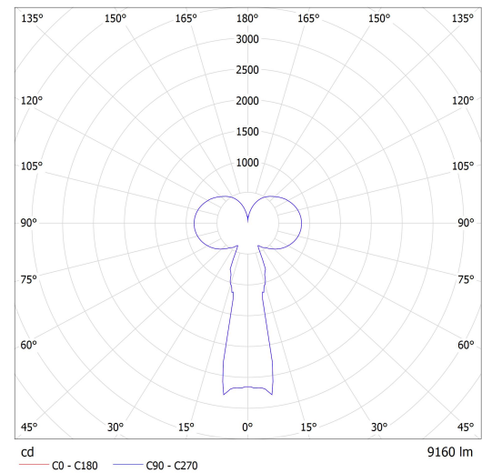
Luminaire: Lucis ZKS.L2A.M620 PA MAIA LED Lamps: 1 x LED G6
