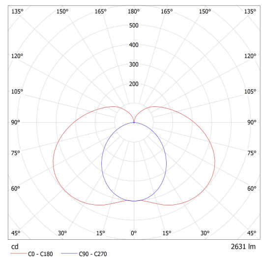
Luminaire: Lucis AU1.L3.1200.X AULA LED Lamps: 1 x LED G6
