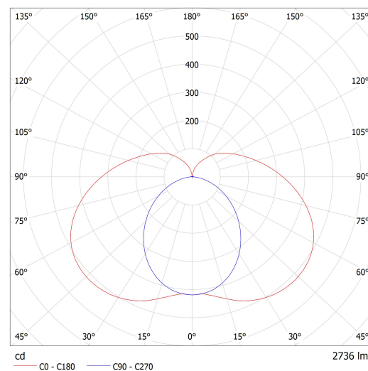
Luminaire: Lucis AU1.L4.1200.X AULA LED Lamps: 1 x LED G6
