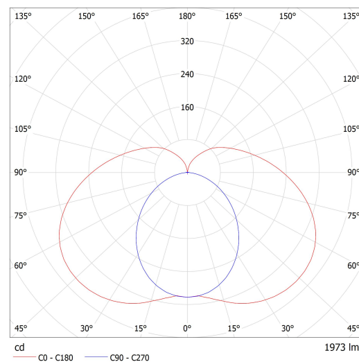
Luminaire: Lucis AU3.L3.900.X AULA LED Lamps: 1 x LED G6
