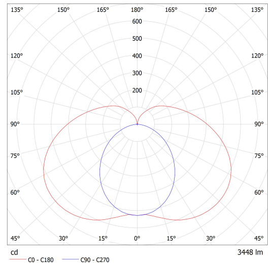
Luminaire: Lucis AU3.L3.1500.X AULA LED Lamps: 1 x LED G6
