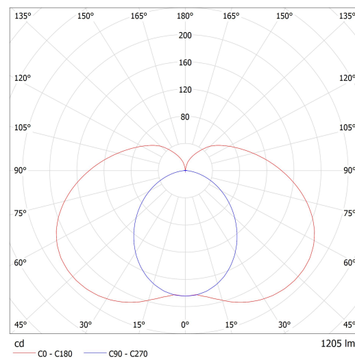
Luminaire: Lucis AU3.L4.600.X AULA LED Lamps: 1 x LED G6
