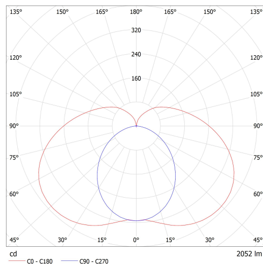
Luminaire: Lucis AU3.L4.900.X AULA LED Lamps: 1 x LED G6
