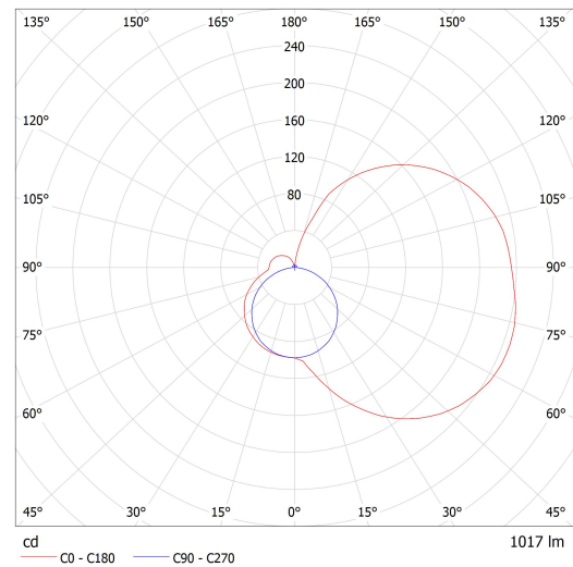
Luminaire: Lucis I1.L3.600.X IZAR I LED Lamps: 1 x LED G6
