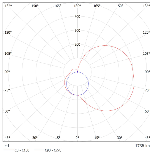
Lucis I1.L3.900.X IZAR I LED / LDC (Polar)
