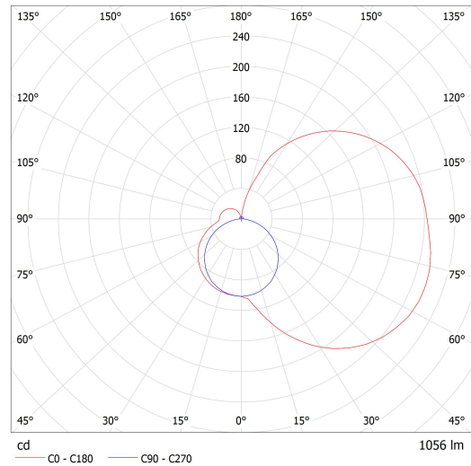
Lucis I1.L4.600.X IZAR I LED / LDC (Polar)
