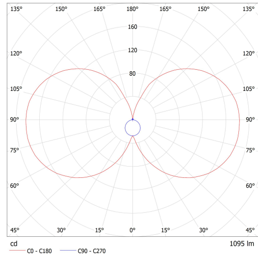
Luminaire: Lucis I2.L3.600.X IZAR II LED Lamps: 1 x LED G6
