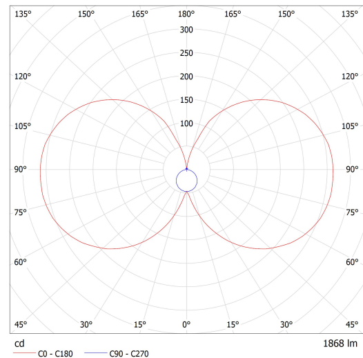
Lucis I2.L3.900.X IZAR II LED / LDC (Polar)
