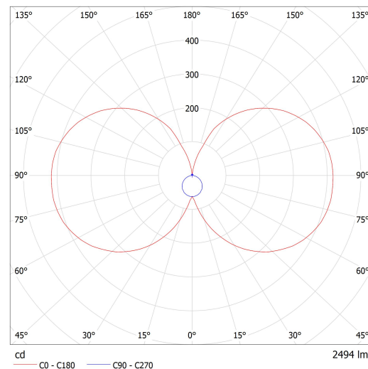
Luminaire: Lucis I2.L3.1200.X IZAR II LED Lamps: 1 x LED G6
