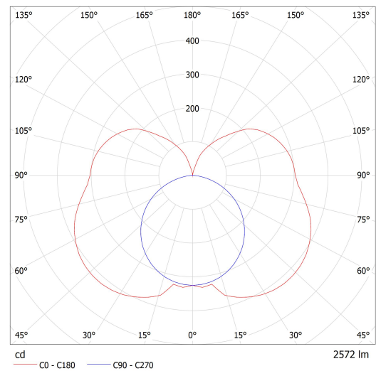
Luminaire: Lucis I3.L3.1200.X IZAR III LED Lamps: 1 x LED G6
