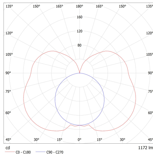
Luminaire: Lucis I3.L4.600.X IZAR III LED Lamps: 1 x LED G6
