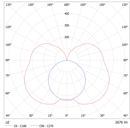
Luminaire: Lucis I3.L4.1200.X IZAR III LED Lamps: 1 x LED G6
