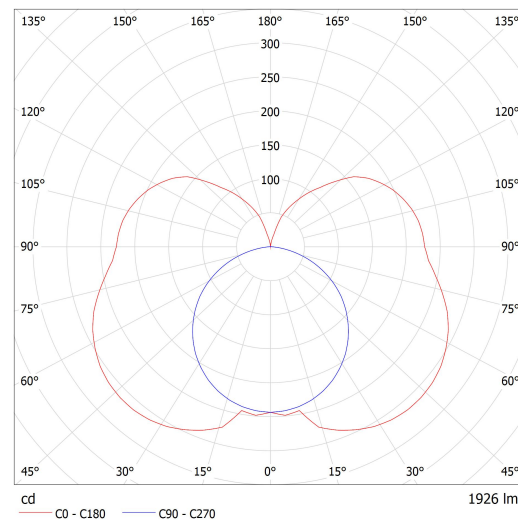
Luminaire: Lucis ZLI3.L3.900.X IZAR III LED Lamps: 1 x LED G6
