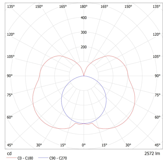
Luminaire: Lucis ZLI3.L3.1200.X IZAR III LED Lamps: 1 x LED G6
