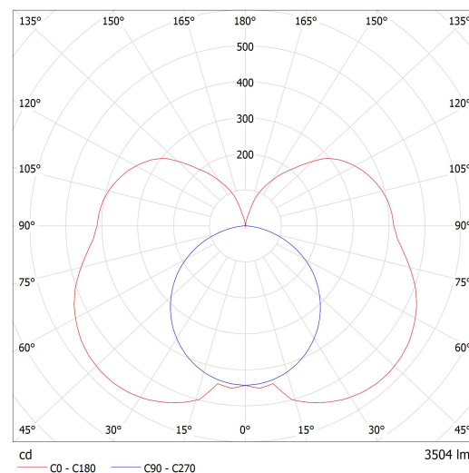
Luminaire: Lucis ZLI3.L4.1500.X IZAR III LED Lamps: 1 x LED G6
