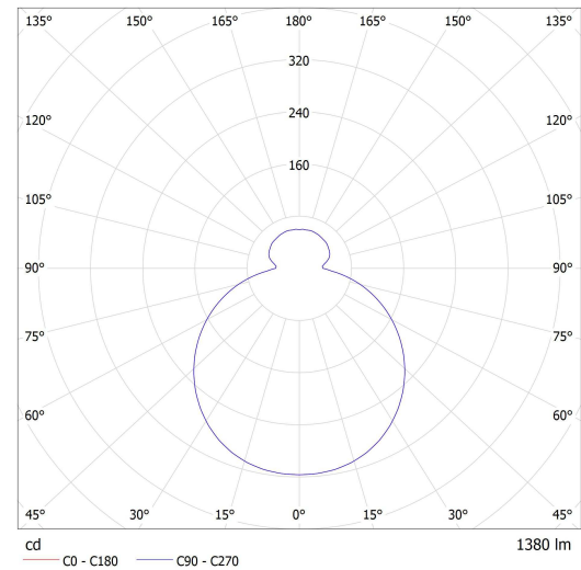
Lucis S24.K2.Z280 ZERO LED / LDC (Polar)
