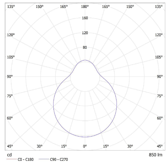
Lucis S19.L2.D280 DAPHNE LED / LDC (Polar)
