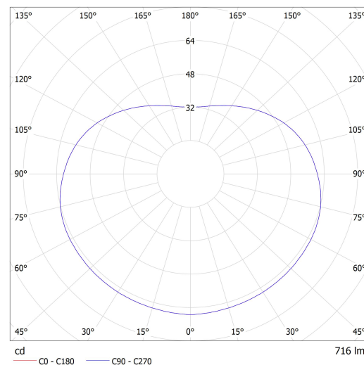
Lucis ZKS.L1.200.X POLARIS ZKS LED / LDC (Polar)
